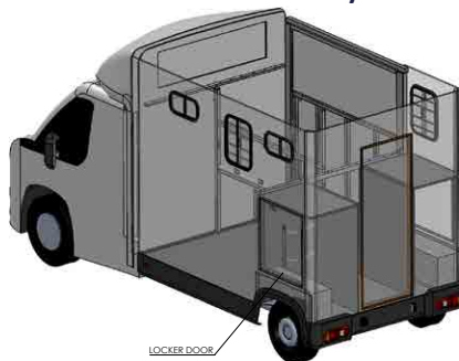
Option 2 (External Tack Lockers)
