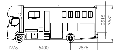
Envoy 4 Stall Layout
