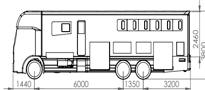
Enterprise 5/6 Stall Layout
