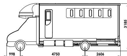
Evolution Transporter Layout
