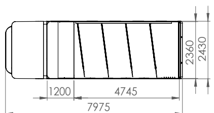
Endeavour Transporter Layout
