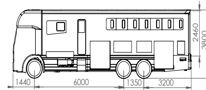
Enterprise 6/7 Stall Layout
