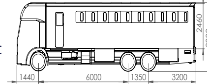
Enterprise Transporter Layout
