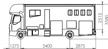
Envoy 3 Stall Layout
