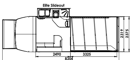
Evolution 3/4 Stall Layout
