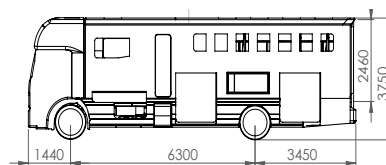
Voyager 4 Stall with Guest Room
