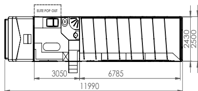
Enterprise 7/8 Stall Layout
