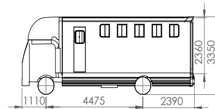
Endeavour Transporter Layout
