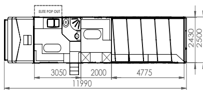
Enterprise 4/5 Stall with Guest Room
