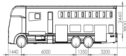
Enterprise 7/8 Stall Layout
