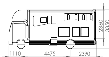
Endeavour 3 Stall Layout
