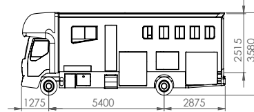
Envoy 2/3 Stall Layout with Guest Room
