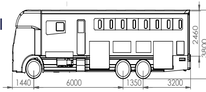
Enterprise 4/5 Stall with Guest Room
