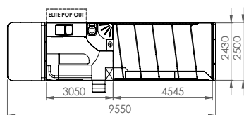
Envoy 5/6 Stall Layout
