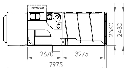
Endeavour 3/4 Stall Layout
